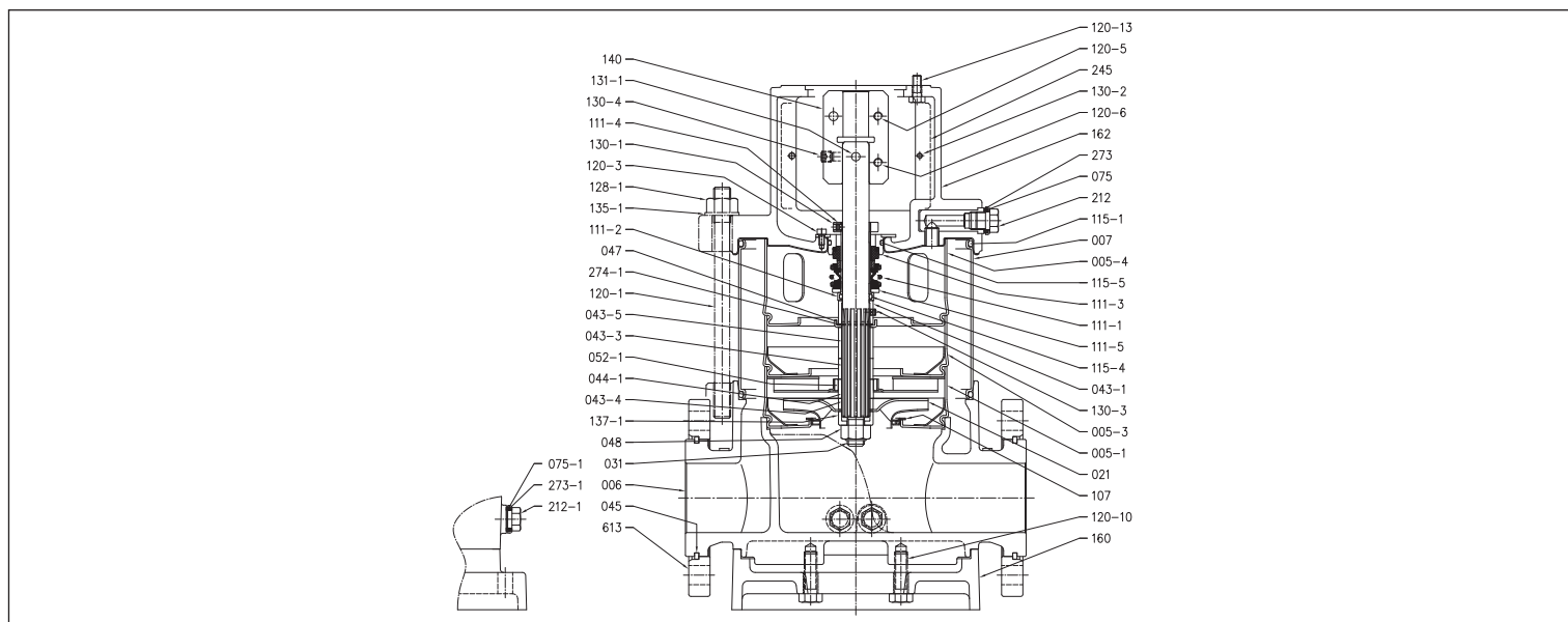
SECTIONAL VIEW EVMG 32 Pump with single ball bearing
